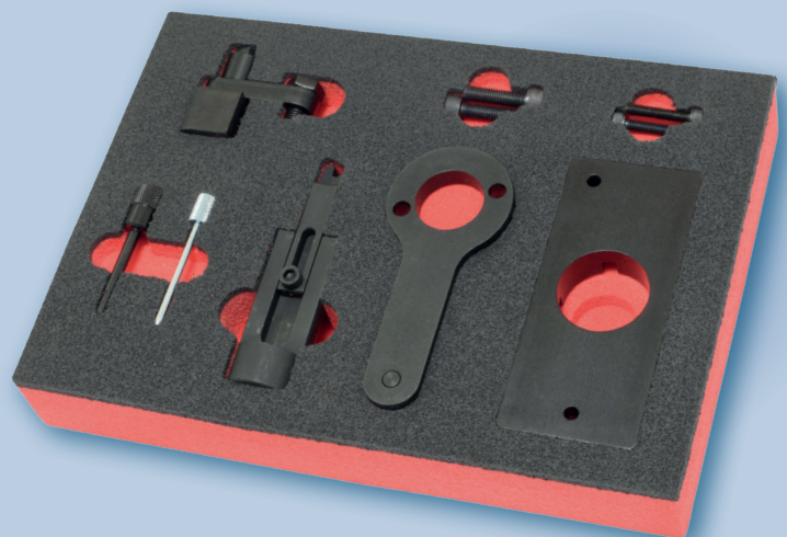
AST5230 DIESEL 2.0 CDTI B20 & D20 (BELT) ENGINE SETTING / LOCKING KIT - OPEL / VAUXHALL
